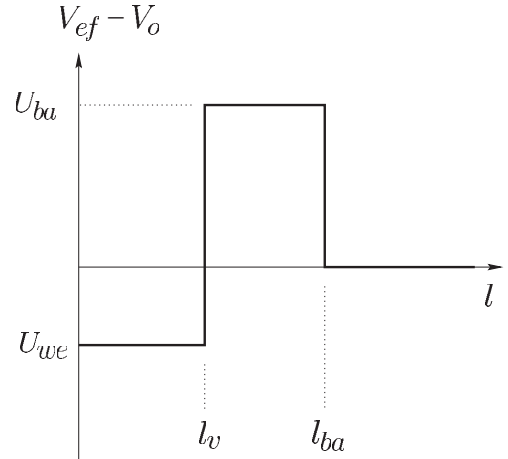
Fig. 6. Schematic form of the effective potential V_{ef} - V_0 defined in (25) as a function of the membrane separation l . The effective potential exhibits i) a potential barrier of height U_{ba} which extends up to the separation l_{ba} , see (24), and ii) a potential well which has the range l_v , arising from the short-ranged sticker potential (23), and the effective depth U_{we} as given by (26).
