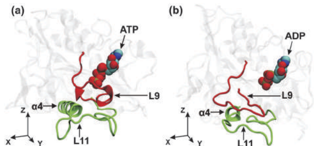
Fig. 6 Kinesin-3 attached to tubulin: dominant conformations of the L9-loop (red) and the L11-loop (green) for (a) the ATP and (b) the ADP states of the motor domain. As before, the (x,y)-plane is tangential to the tubulin surface and the y-axis is parallel to the long principal axis of the \alpha 4 -helix in the ATP state. Comparison of the two conformations reveals that the \gamma -phosphate release from the nucleotide binding pocket causes the L9-loop to move away from the nucleotide, to change its interaction pattern with the L11-loop, see the corresponding atomic separations as described in Fig. 7 below, and to induce a rotation of the \alpha 4 -helix within the (x,y)-plane as in Fig. 5(b).
